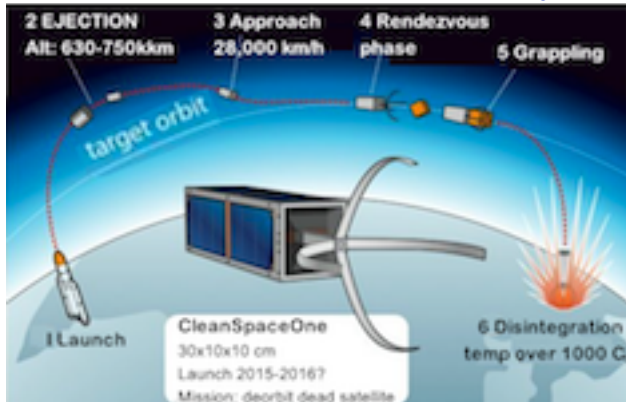
Swiss CleanSpace One spacecraft (above)
